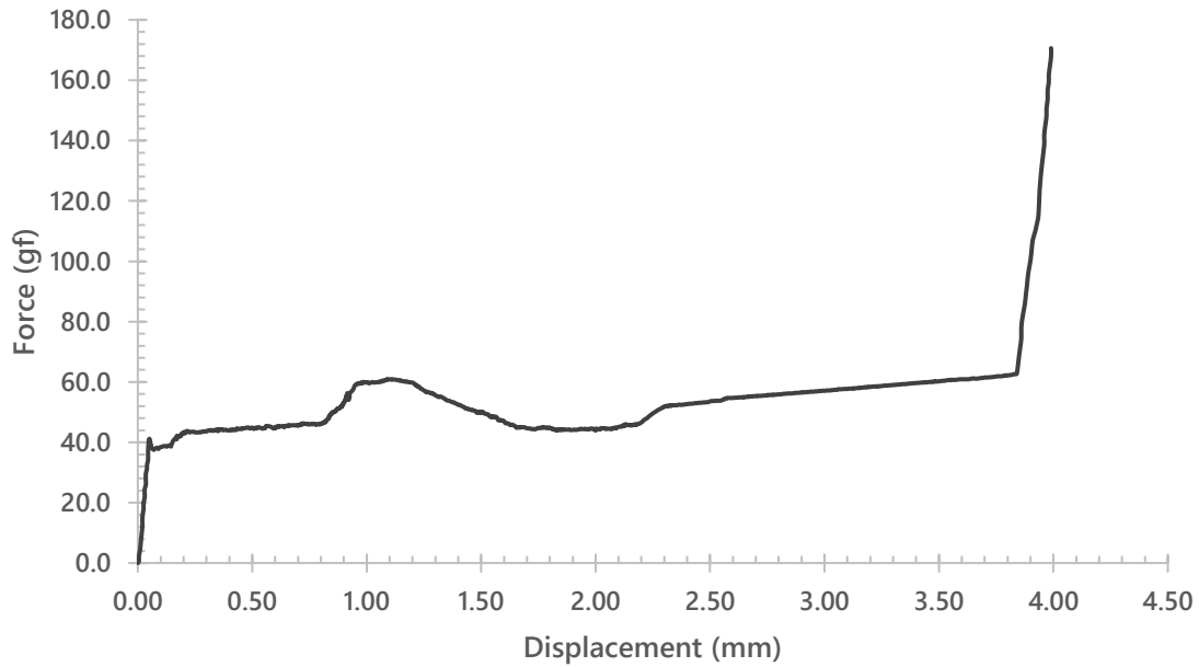
Cherry MX Lumina Brown (Upstroke)
